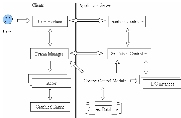
Figure 1. Basic Architecture for iTV Storytelling
